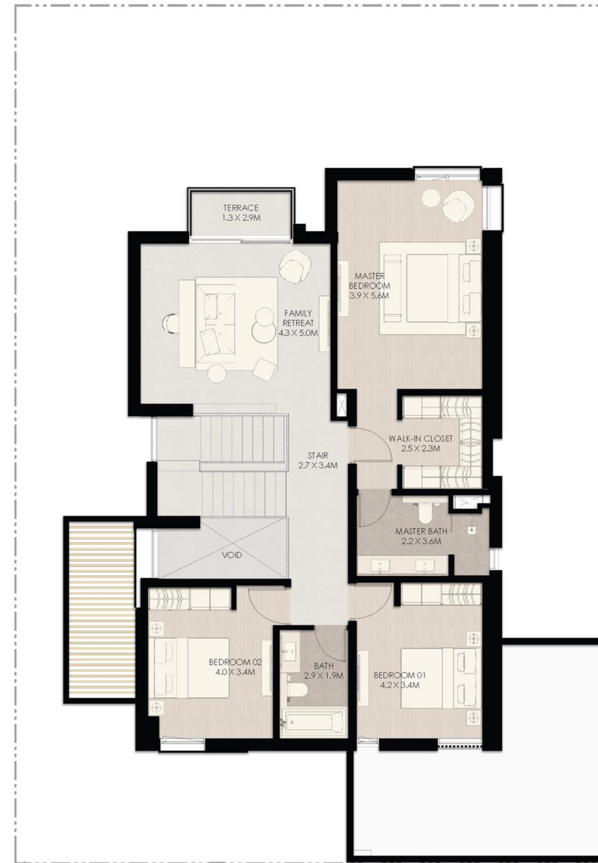
FIRST FLOOR
